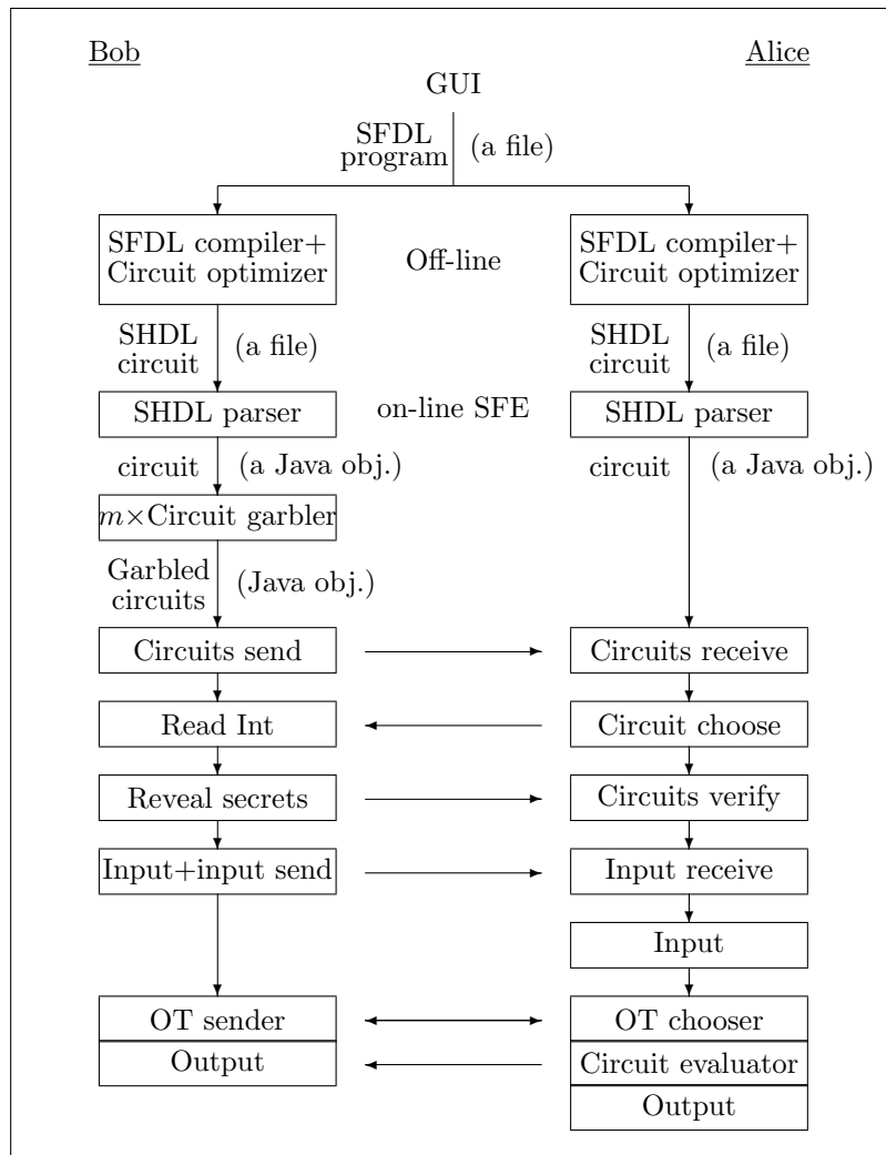
Figure 1: Computation overview
